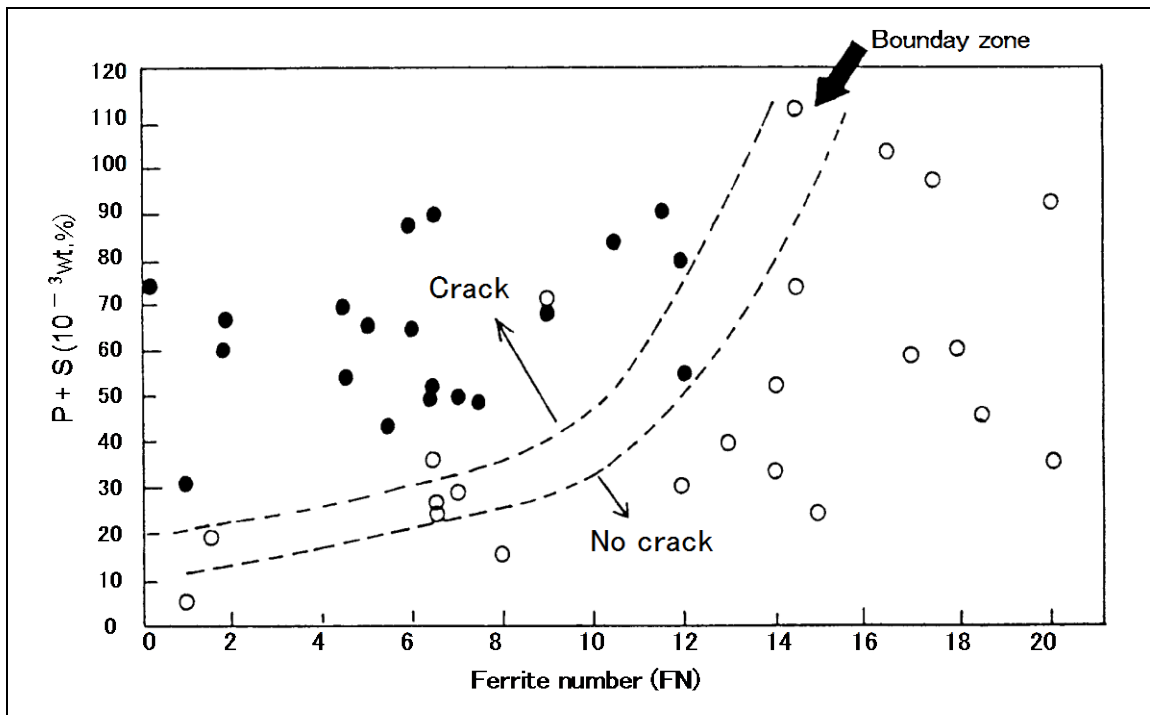
Fig. 2.6 — Effects of P+S content and ferrite number on hot crack susceptibility of Type 309 weld metals
