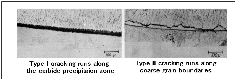
Photo 4.2 — Typical cracks occurred in the vicinity of the transition zone of the austenitic stainless steel weld cladded on a low-alloy base metal
