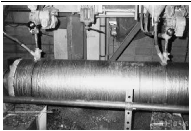
Photo 8.4 — SAW with a martensitic type flux-cored wire (US-H600N) and a fused flux (MF-30), hardfacing a steel mill roller
