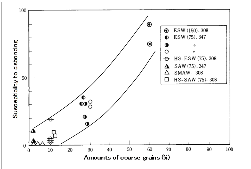
Fig. 4.9 — Susceptibility to the disbonding of cladded austenitic stainless steel weld metals as a function of the amount of coarse grains •The figures entered in the parentheses indicate the width of strip electrodes •308 and 347 indicate the types of cladded weld metals •ESW: electroslag welding; HS-ESW: high-speed ESW; SAW: submerged arc welding; SMAW: shielded metal arc welding; HS-SAW: high-speed SAW
