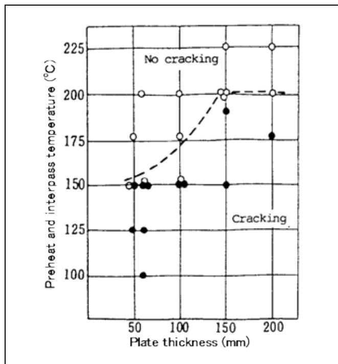
Fig. 2.6 — Crack test results of restrained 2.25Cr-1Mo steel welds by submerged arc welding
